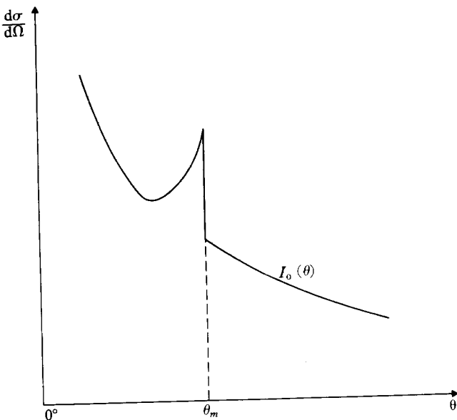
13.6 Schematic diagram of the differential cross-section for the elastic scattering of one atom by another showing the classical rainbow effect of equation [13.44].
